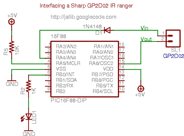
Figure 8: Interfacing Sharp GP2D02 IR range : schematic
