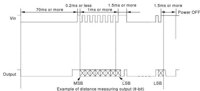
Figure 7: GD2D02 IR ranger : timing chart
