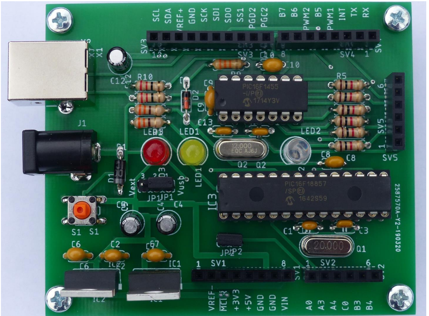
JALPIC One development board
